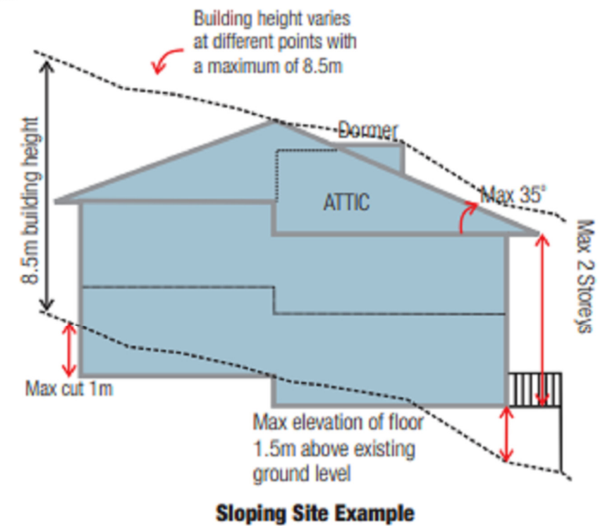
Figure 3.1(a) Explanation of building height controls (I)
