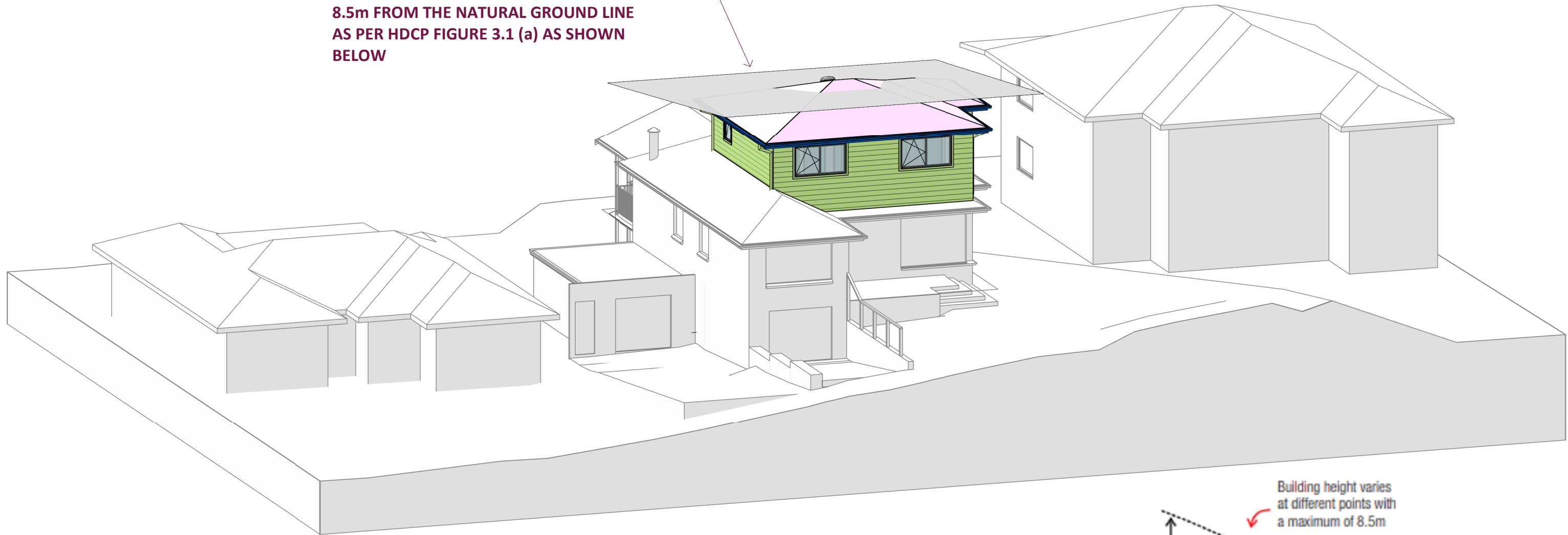
3D HEIGHT PLANE DIAGRAM
