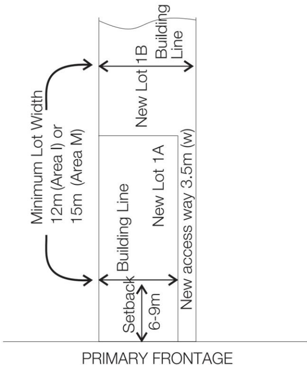
Figure 6.2-b-6.2(b): Minimum lot width required for all allotments. (l)
