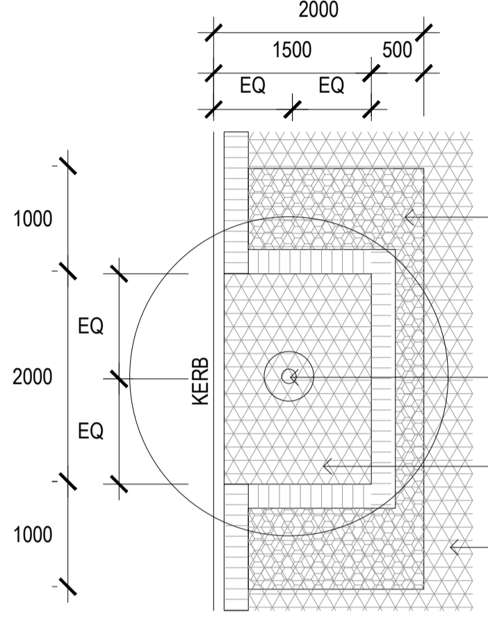
DETAIL 01 STREET TREE SCALE 1:50
