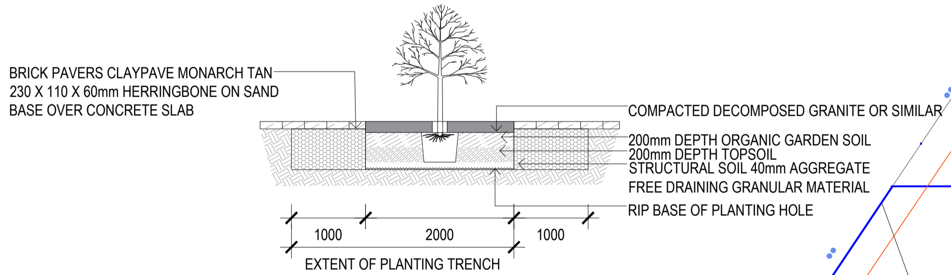
DETAIL 03 STREET TREE SCALE 1:50
