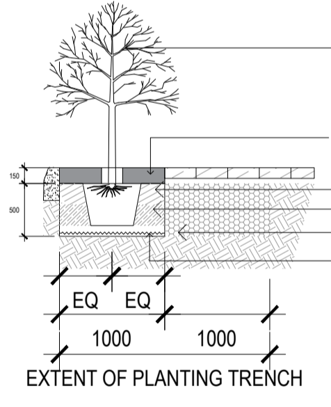
DETAIL 02 STREET TREE SCALE 1:50
